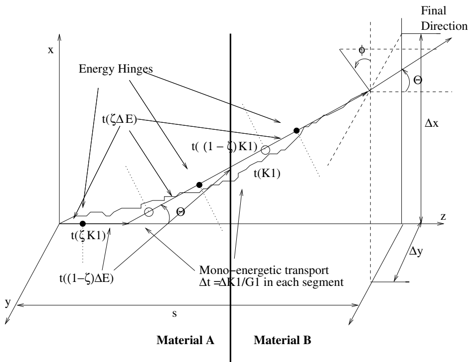
Figure 2.12: Electron transport across region boundaries.
