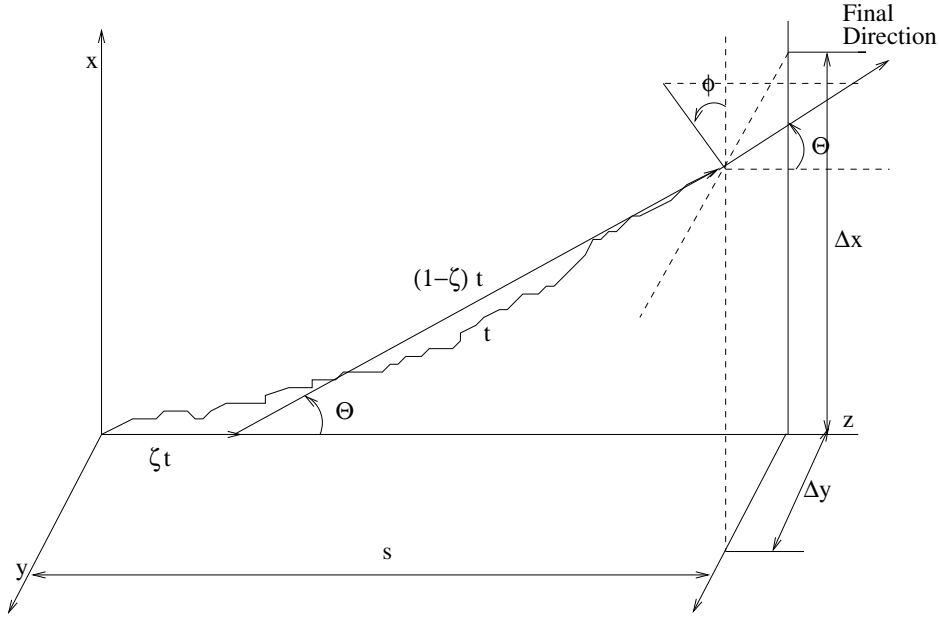
Figure 2.9: Random hinge transport mechanics schematic.
