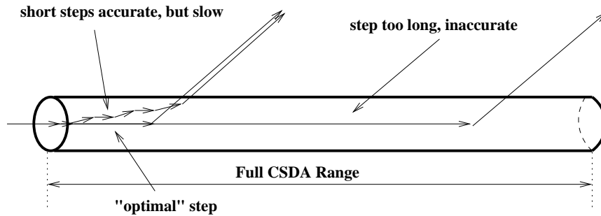
Figure 2.15: Schematic illustrating the “broomstick” problem.
