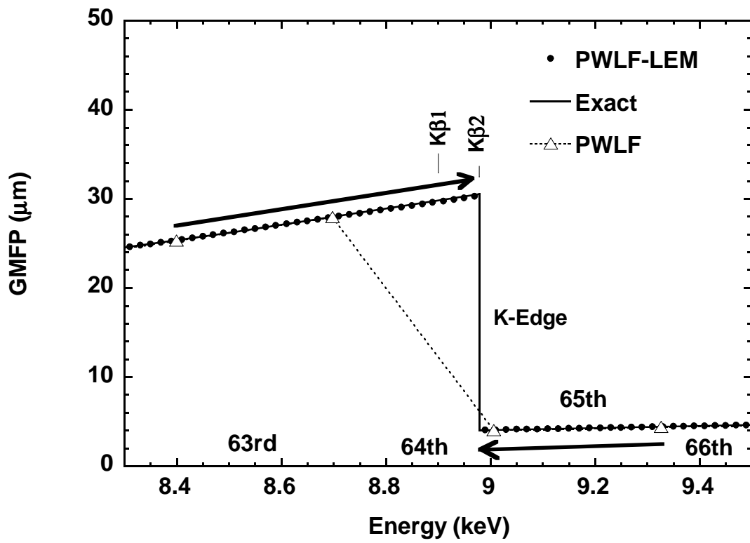
Figure 2.21: Cu GMFP values evaluated by PWLF and LEM
