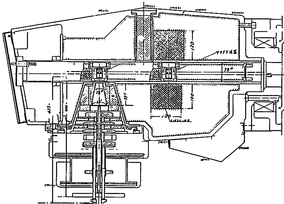
Fig.1 Cutaway view of Shimadzu RTGS-2 telecobalt therapy unit. (courtesy of Shimadzu Co.)
